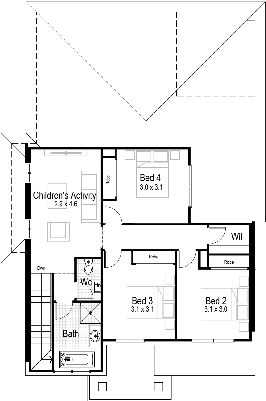
First Floor
